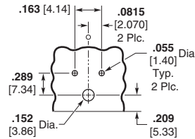
2 Circuit, In-Line
