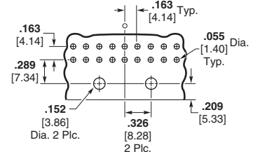
14 and 18 Circuit, Dual Row
