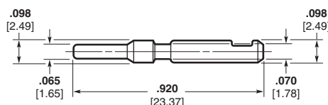
Part Number 794369-1
